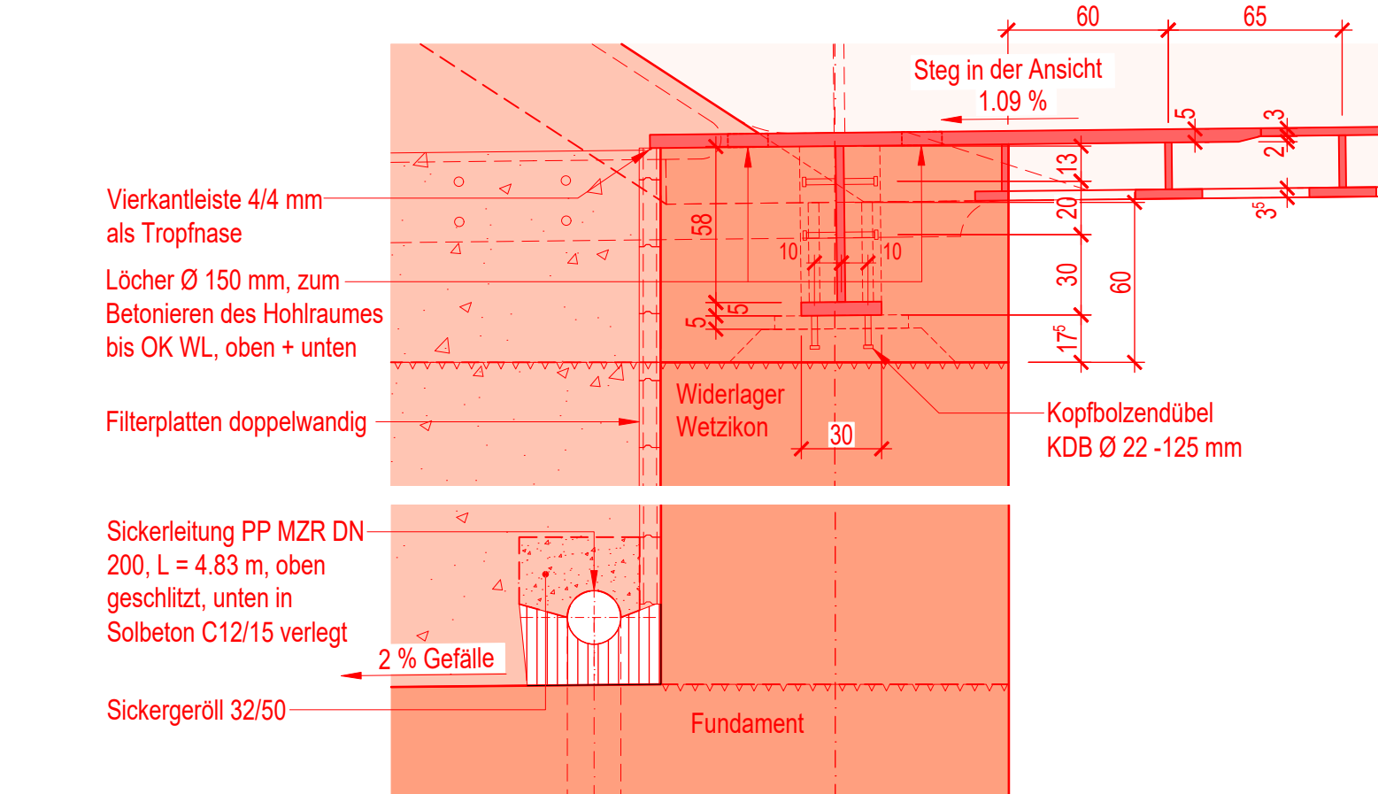
Detail -B-, 1 : 25
